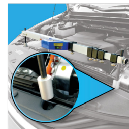
DF3TCAS DentFix Self Centering Tips for DentFix Tram Gauge
